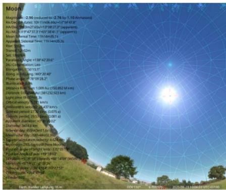
Figure 2. Display Position Sun at Conjunction August 23 , 2025, at 1:06:22 PM WIB. Results of the Stellarium Simulation in Bandar Lampung.
