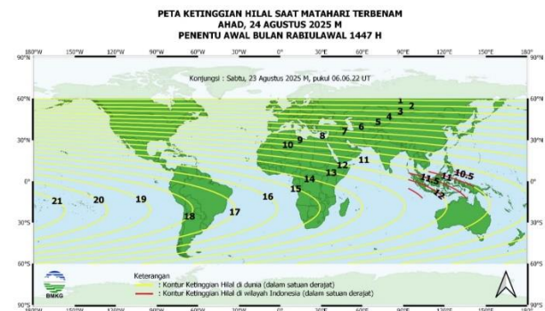
Figure 4. Map of the Crescent Height for observers between 60^\circ\text{N} to 60^\circ\text{S} on Sunday, August 24, 2025 AD
